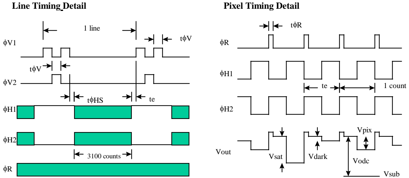
Figure 6: Line Timing
